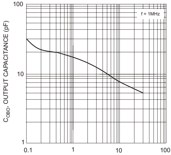
V CB , COLLECTOR-BASE VOLTAGE (V) Fig. 3, Output Capacitance vs. Collector-Base Voltage
