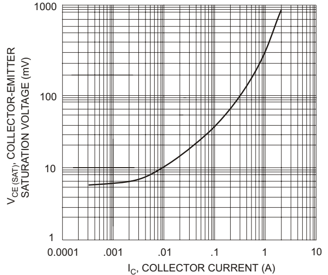
I C , COLLECTOR CURRENT (A) Fig. 4, Collector Saturation Voltage vs Collector Current
